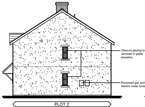
EAST ELEVATION
